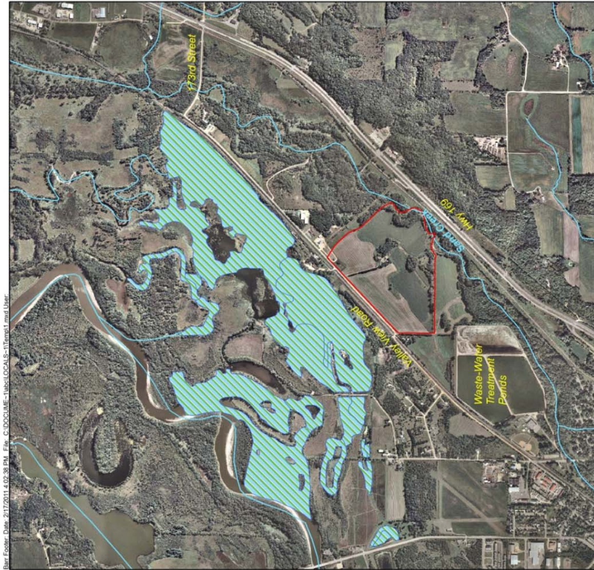
Figure 3-8 POTENTIAL GROUNDWATER-INFLUENCED WETLANDS Jordan Aggregates EIS Scott County, Minnesota
